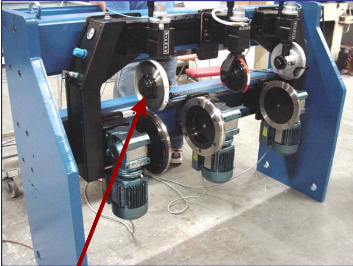
Edge trim blade bevels outward with anvil knife support under web.
